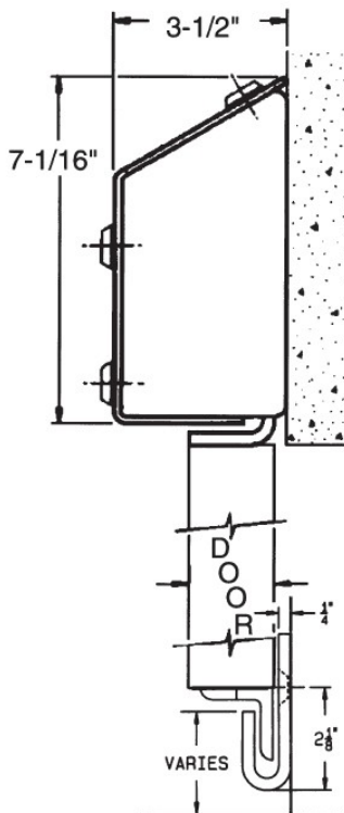
Masonry installation
